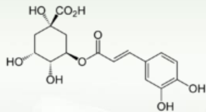
Chlorogenic acid
